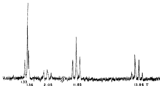
Figure 1. Nmr spectrum of trans -15,16-diethyldihydropyrene, measured in deuterochloroform solution using a Varian A-60 spectrometer.
